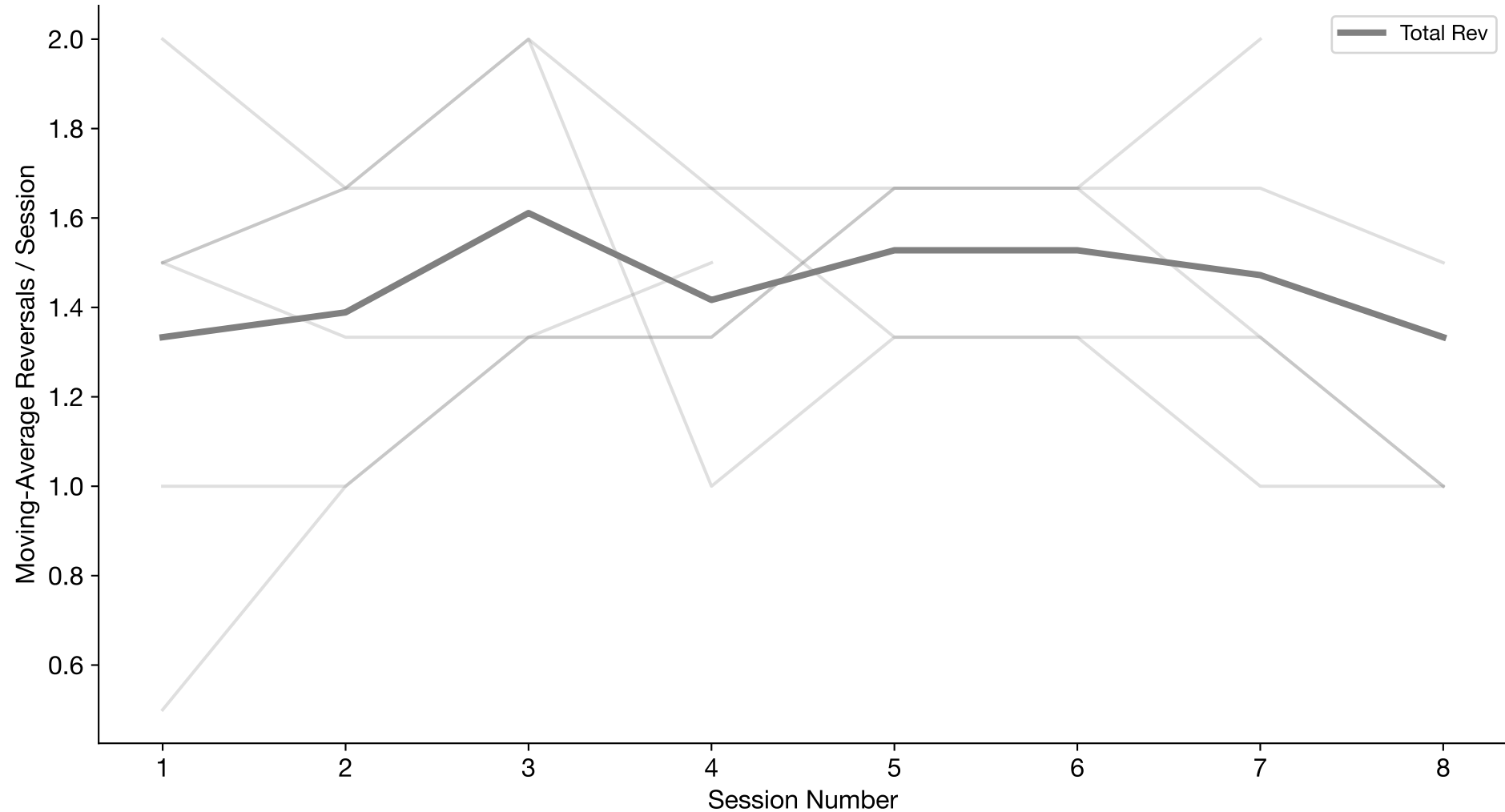
Moving-Average Total Reversals Over Time (n=6 subjects; sessions per subject=4–8; window=3)
